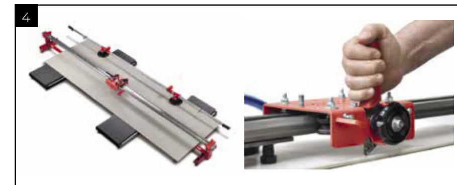
4. Guide with cutting carriage
